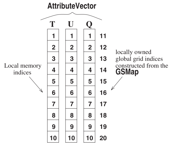
Fig. 3 Relationship between local memory indices in an AttributeVector and the grid point numbering contained in the GSM ap for the points owned by processor 1 in Figure 2. In this example, the AV ect is being used to store three variables: temperature ( T ), east-west velocity ( U ), and specific humidity ( Q ).
