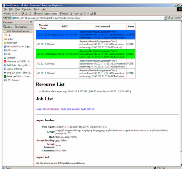
Figure 5. Status of jobs maintained as part of the virtual machine manager for a sporadic Grid.
