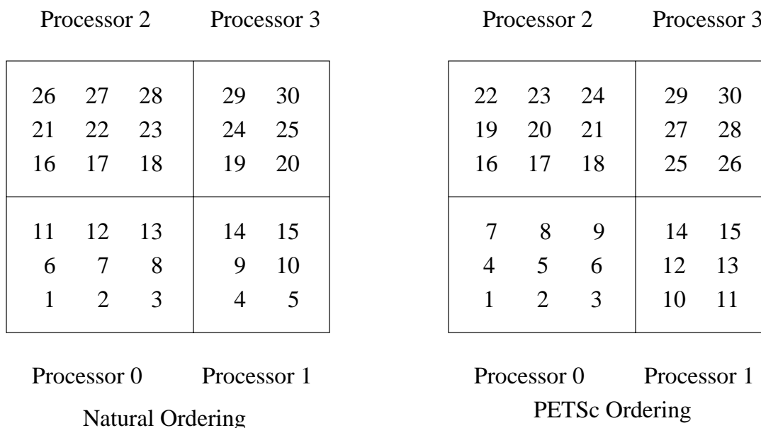
Fig. 2.2: Natural Ordering and PETSc Ordering for a 2D Distributed Array (Four Processes)
