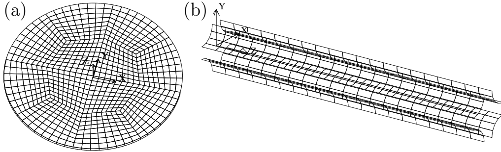
Fig. 1. Tensor-product mesh examples for Rayleigh-Bénard convection (a) and reactor core cooling (b).
