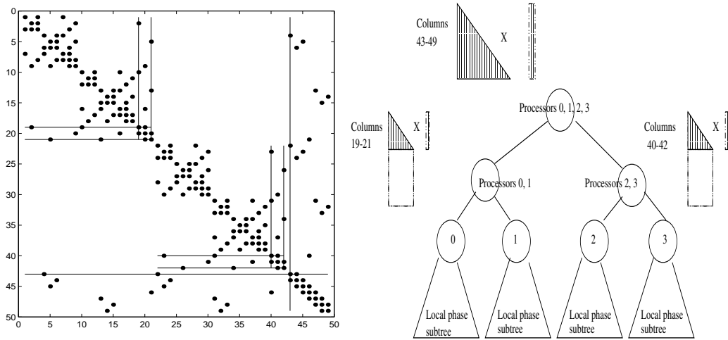
Fig. 2. Structure of L + L^T associated with the matrix of a 7 \times 7 five-point finite-difference grid ordered using nested dissection (left). Forward triangular solution is shown using 4 processors 0, \dots, 3 (right). Shaded triangular submatrices are inverted once to replace distributed substitution by matrix-vector multiplication in subsequent triangular solutions.
