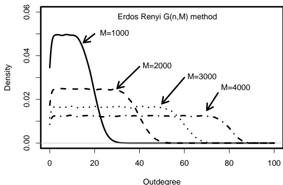
Figure 7: Distribution of out-degrees of graphs generated using G(n, M) for different number of edges.
