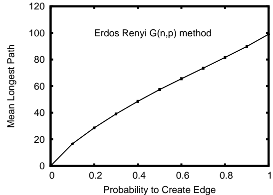
Figure 1: Mean longest path length of graphs generated using G(n, p) for different probabilities.
