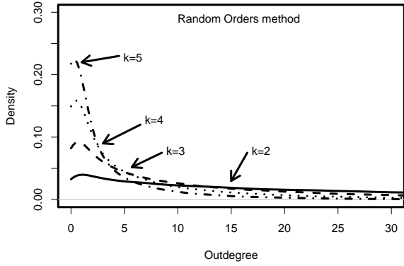
Figure 10: Distribution of out-degrees of graphs generated using Random Orders for different number of intersected total orders.
