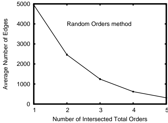
Figure 14: Average number of edges of graphs generated using Random Orders for different number of intersected total orders.
