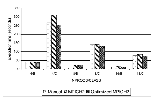
Fig. 5. Execution time of the NAS MG benchmark on jazz (left) and on sunwolf (right)
