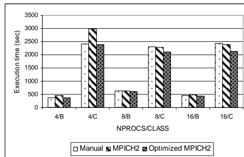
Fig. 6. Execution time of the NAS MG benchmark on sunwolf
